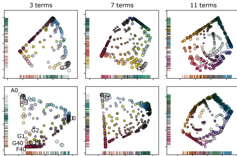
Fig. 1: Six languages from the WCS differing in the number of terms (columns). Rug plots display the distribution of terms within the 2D space. The size of the points represents agreement for the color term within the language.
